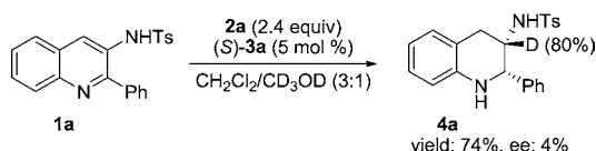
Scheme 6. Isotopic Labeling Experiment
